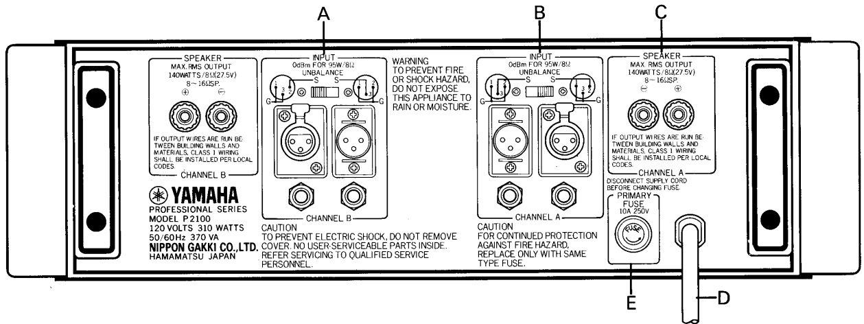
Fig. 2 – P2100 Rear Panel**
