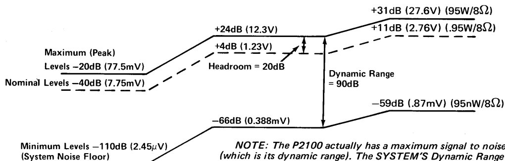
Fig. 33 – Dynamic Range in an Audio System
