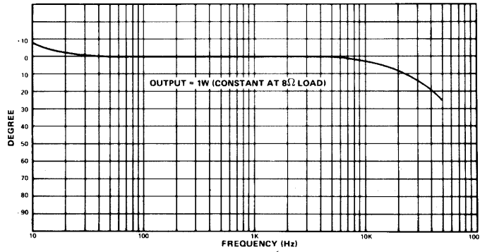
Fig. 12 - Phase Response vs Frequency
