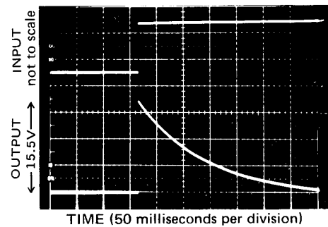
Fig. 27 - Unit-step Function Response
