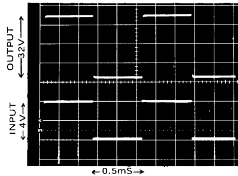
Fig. 26 - Square-Wave Response into a Highly-Inductive Load (at 1kHz) The P2100's ability to maintain a sharply defined square wave output into a reactive load demonstrates stability under the worst conditions. There is still a complete lack of unwanted ringing, as well as virtually unmeasurable phase shift.
