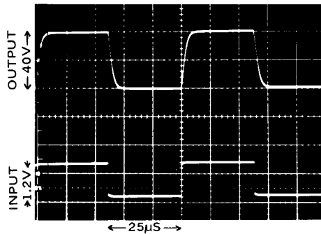
Fig. 23 - 20,000 Hz Square-Wave Response The extremely fast and symmetrical rise and fall times of the amplifier are evident, demonstrating the ability to reproduce accurately musical waveforms and harmonics well beyond the range of human hearing.
