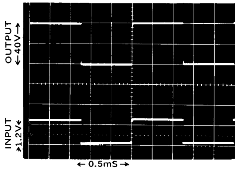
Fig. 22 - 1,000Hz Square-Wave Response Near perfect response is evident in the duplication of the input waveform by the output waveform. There are no "squiggles" or spikes, meaning there is no ringing or overshoot.
