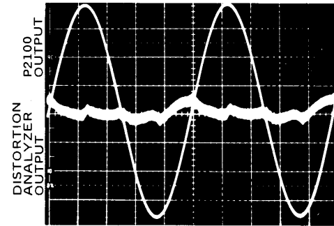
Fig. 25 - 20,000Hz Sine Wave, Shown with Highly-Magnified Noise & Distortion Components Even at 20kHz, the P2100 produces 95 watts continuous output with low distortion and symmetrical reproduction. As in Fig. 11, the noise (magnified here) is actually some 110dB below the sine wave.
