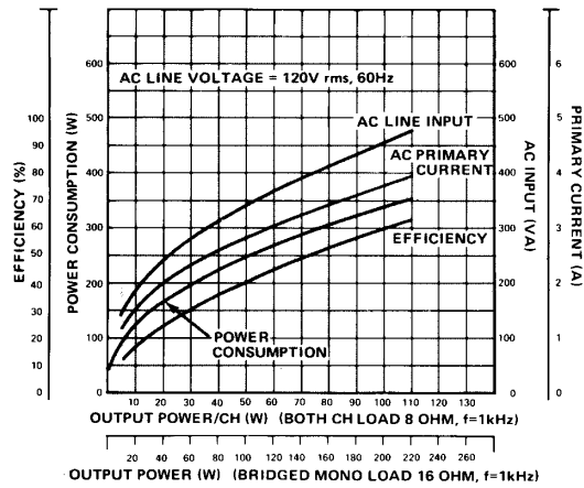
Fig. 13 - Power Consumption
