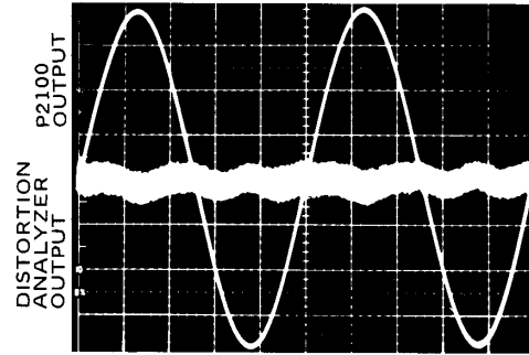
Fig. 24 - 1,000Hz Sine Wave, Shows with Highly Magnified Noise & Distortion Components Even at full 95 watt output (8 ohms), the P2100's distortion is so low that it is almost buried in the noise, which is some 110dB below the sine wave output. The sine wave is clean and symmetrical.
