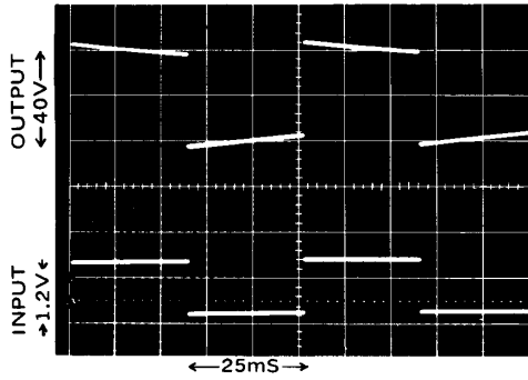
Fig. 21 - 20Hz Square-Wave Response The output waveform displays very respectable low frequency response. The slight tilt shows a DC gain of unity, which prevents damage to speakers in the event any DC offset is fed to the amplifier input.
